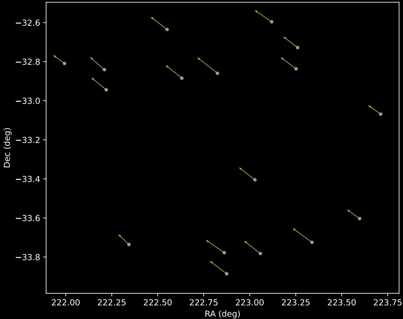
APOGEE DR17 Cluster 16 Proper Motion Vectors (n=17)
