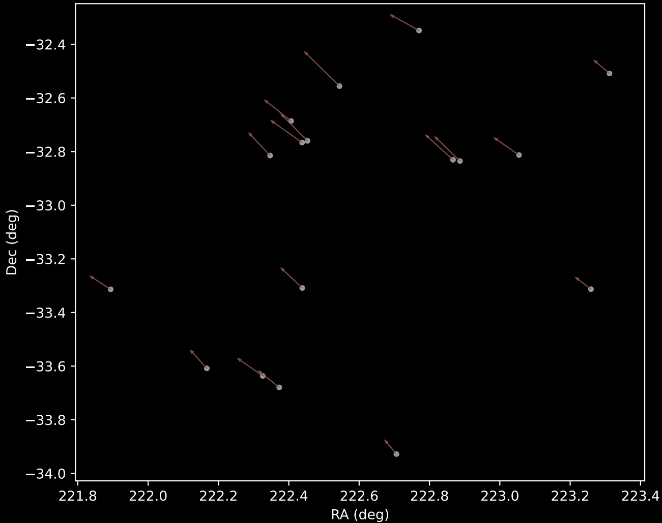
APOGEE DR17 Cluster 10 Proper Motion Vectors (n=17)
