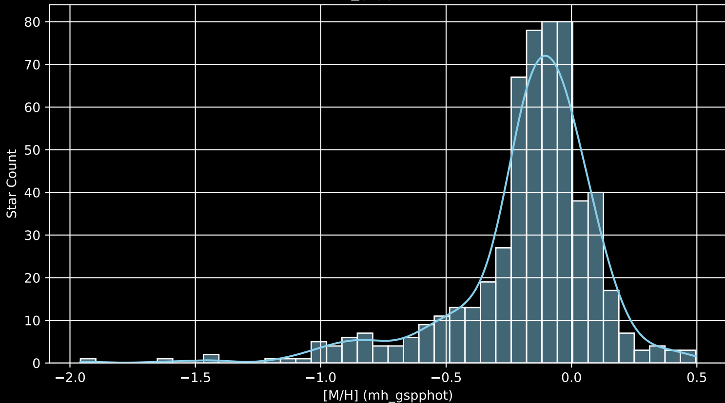
APOGEE DR17 Field: [251+00 [M/H] (mh_gspphot) (n= 555)
