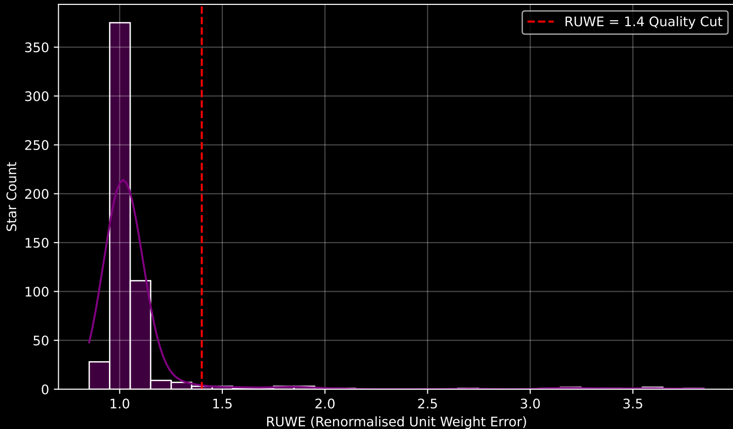
GAPOGEE DR17 Field [251+00] RUWE Distribution (n= 553)
