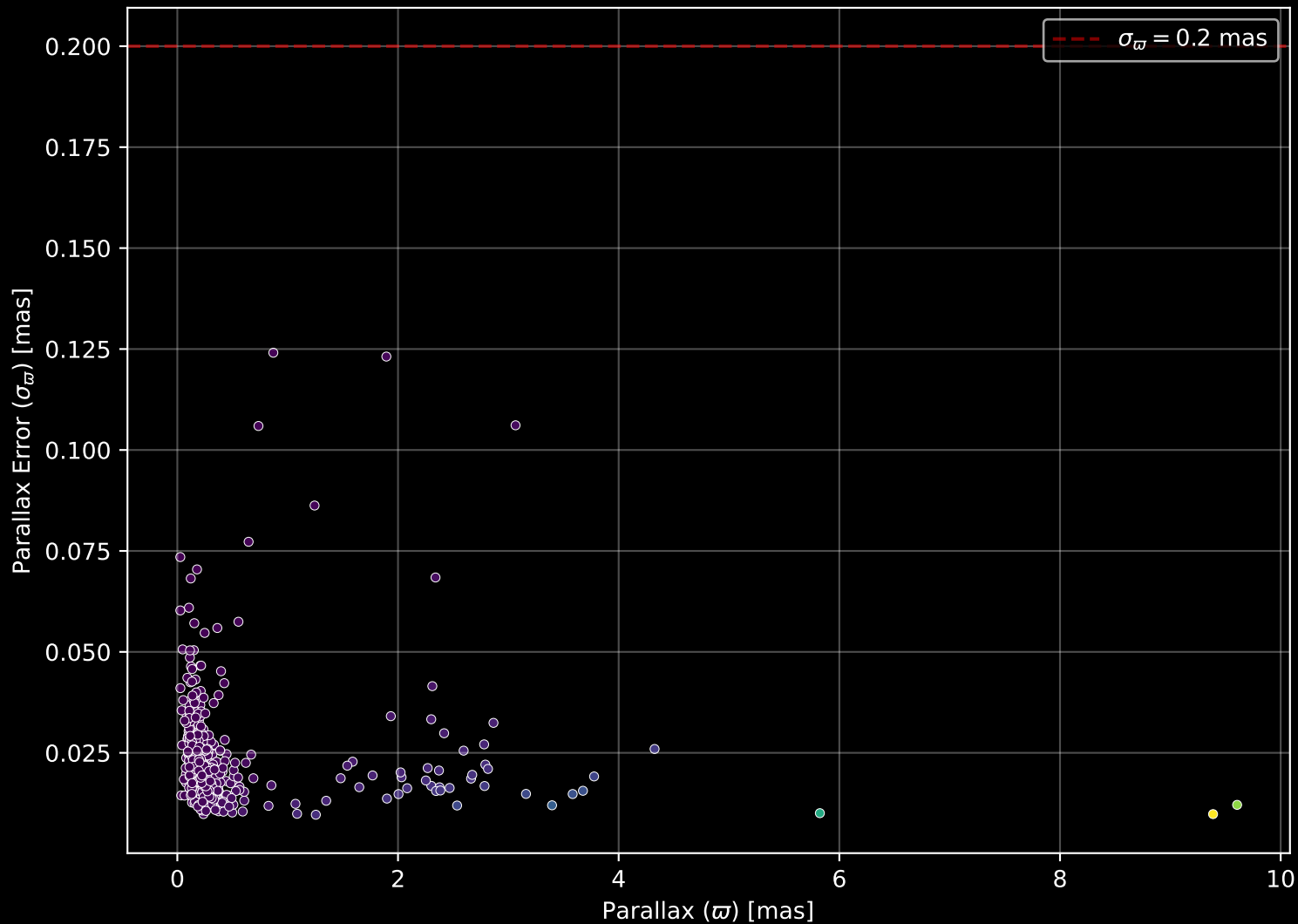
APOGEE DR17 Field: [251+00] Parallax Quality (n= 559)
