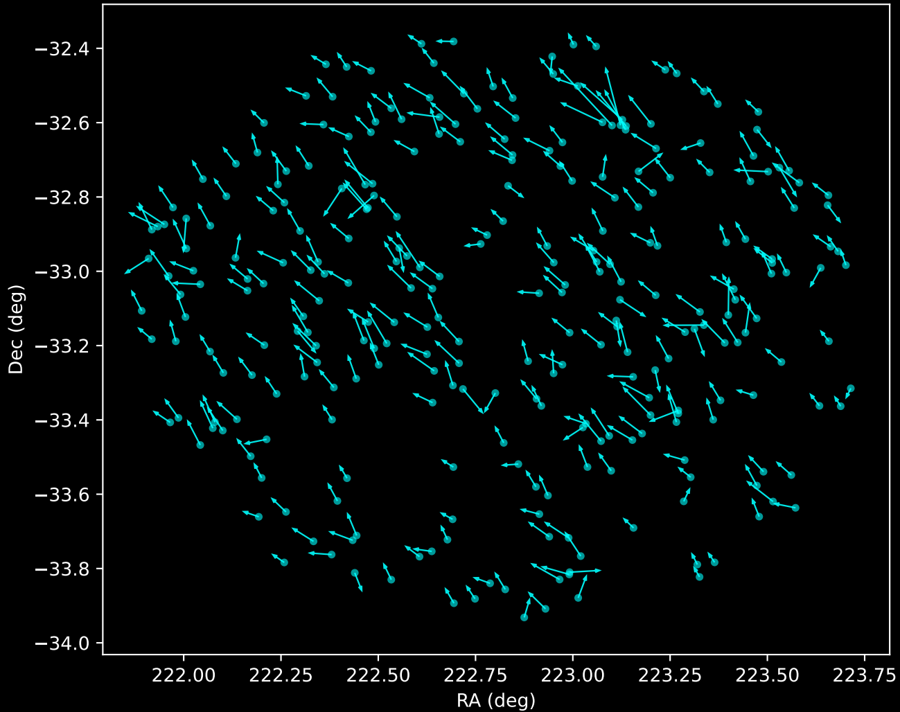
APOGEE DR17 Noise Stream Proper Motion Vectors (n=281)
