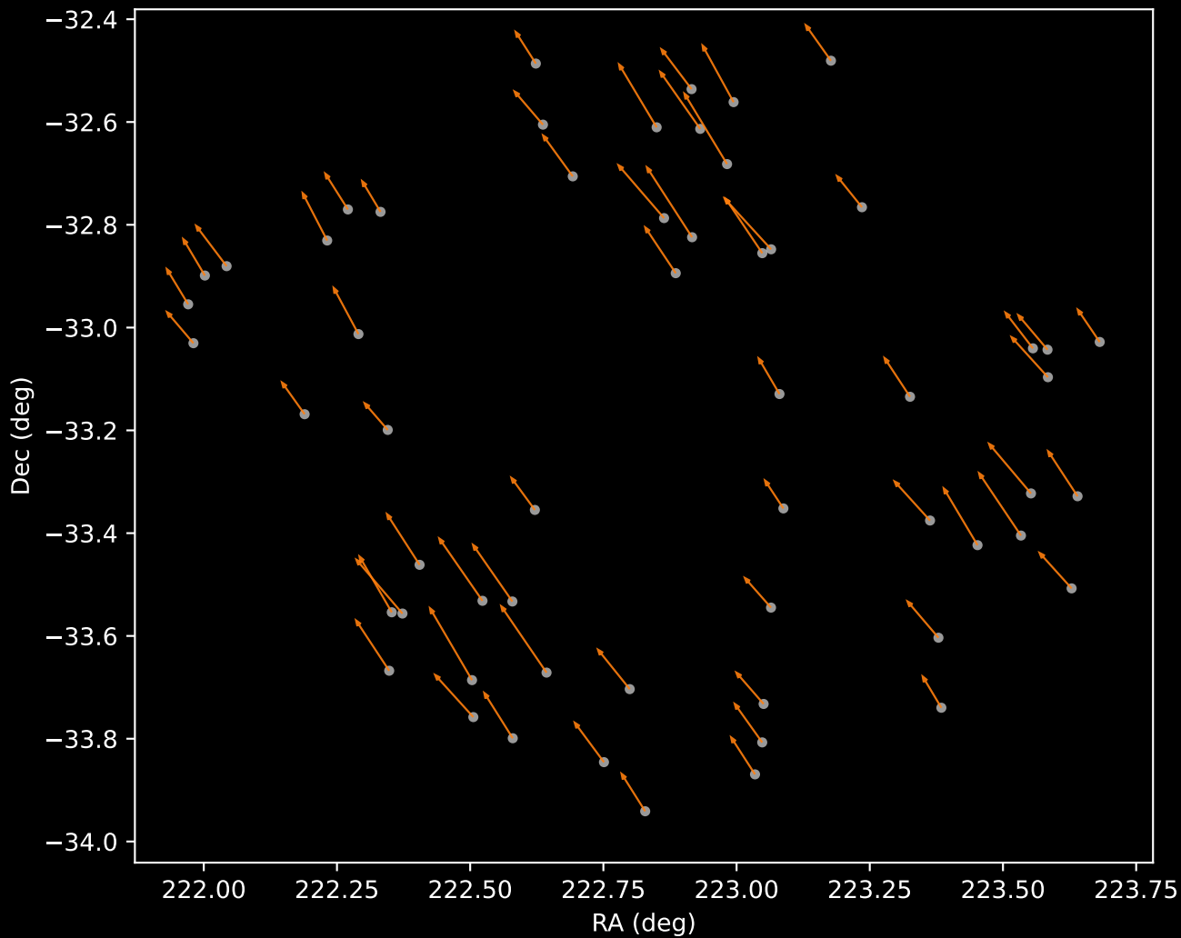
APOGEE DR17 Cluster 22 Proper Motion Vectors (n=58)
