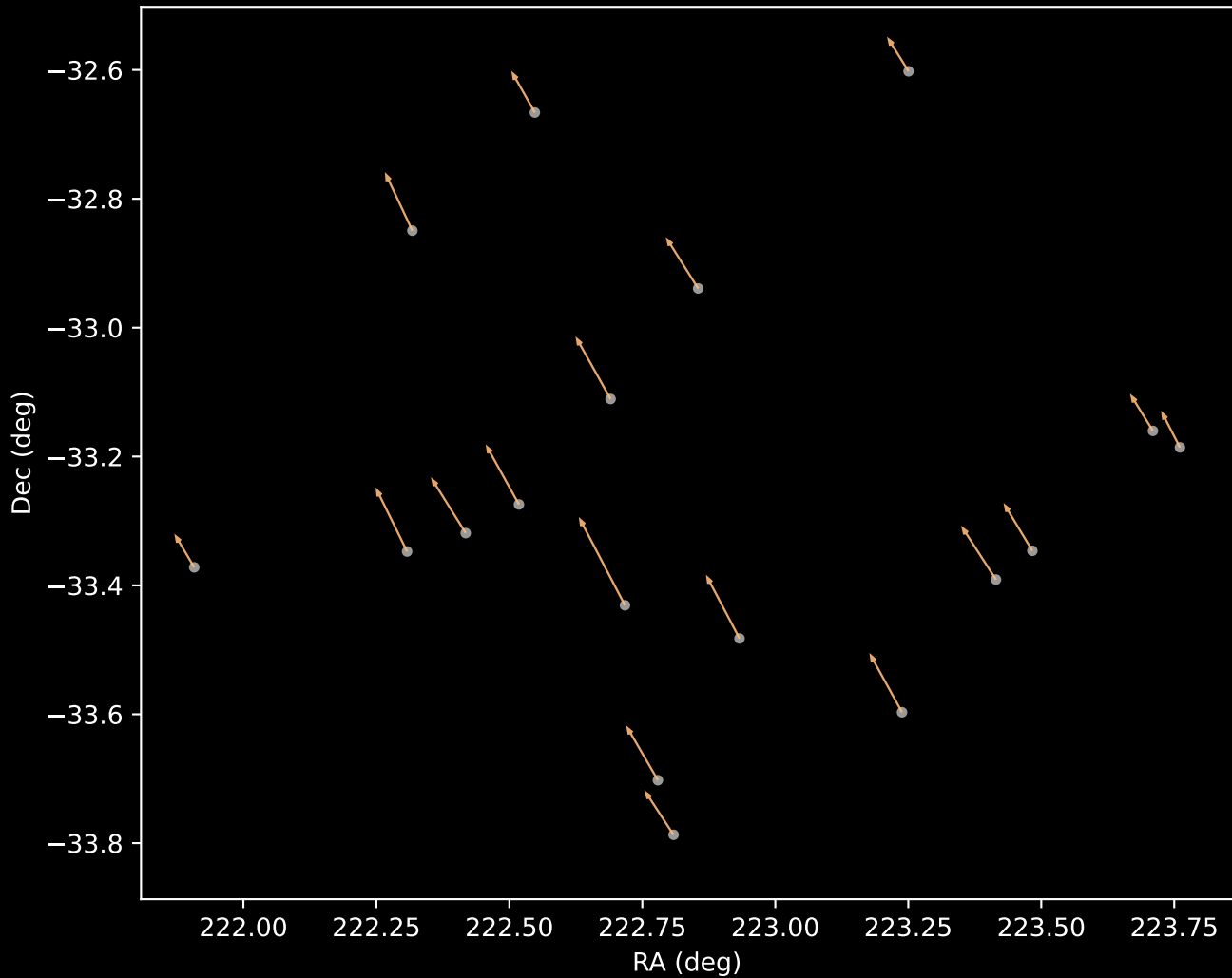
APOGEE DR17 Cluster 23 Proper Motion Vectors (n=18)
