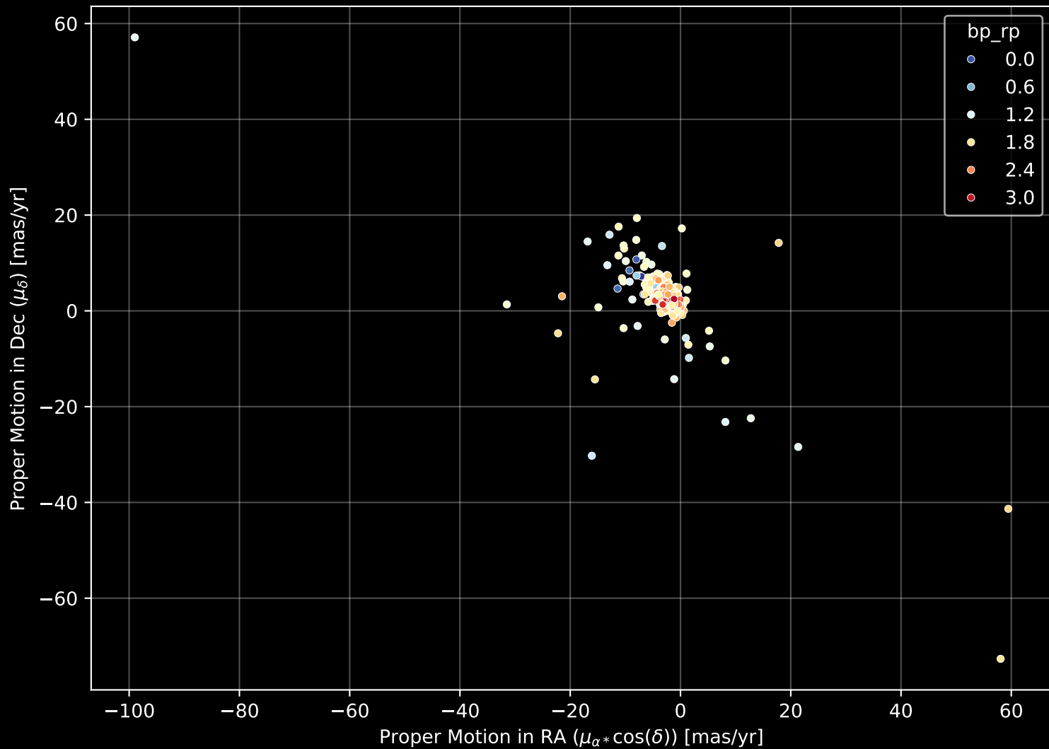
APOGEE DR17 Field: [251+00] Proper Motion Diagram (n= 559)
