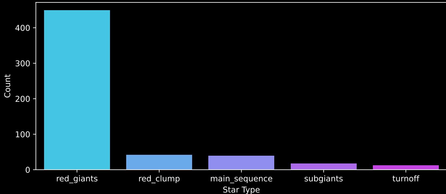
APOGEE DR17 Field: [251+00] Count plot of Star Type
